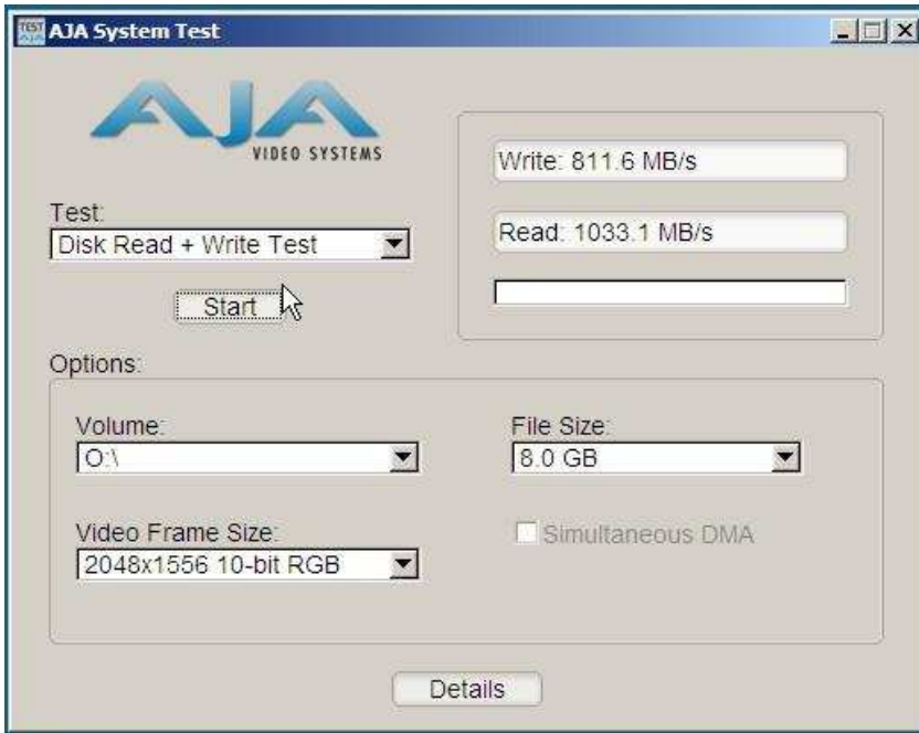
AJA system test showing 811.6MB/s write and 1033.1 MB/s disk read for 2048x1556 10-bit RGB video frames with 8GB files size.
