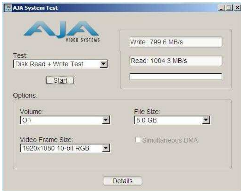
AJA system test showing 799.6MB/s write and 1004.3 MB/s disk read for 1920x1080 10-bit RGB video frames with 8GB files size.
