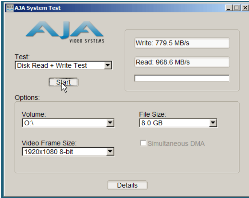
AJA system test showing 779.5MB/s write and 968.6 MB/s disk read for 1920x1080 8-bit video frames with 8GB files size.
